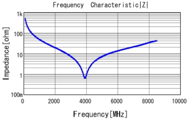
GRM1885C1H3R1CA01 |Z| DCOV, 25degC
