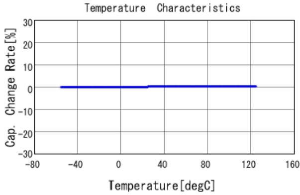
GRM1885C1H3R1CA01 C-Temp. capchange, DCOV, AC1Vrms
