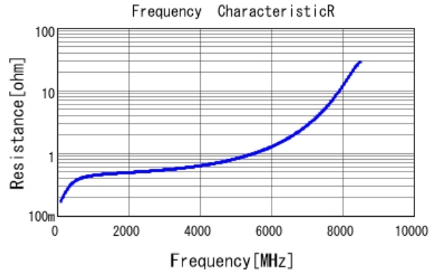
GRM1885C1H3R1CA01 R DCOV, 25degC
