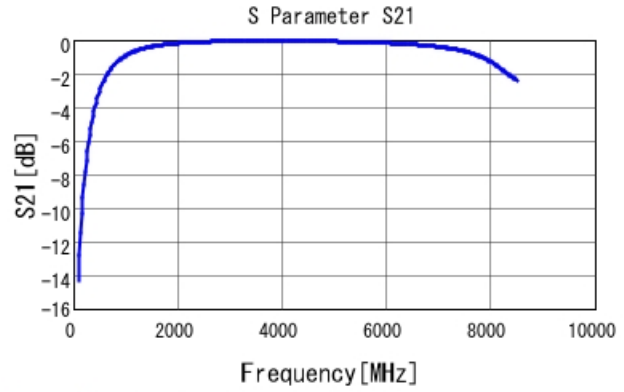
GRM1885C1H3R1CA01 S21 DCOV, 25degC
