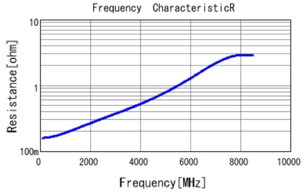
GCM0335C1E180JA16 R DC0V, 25degC
