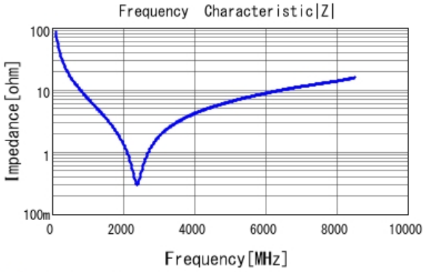
GCM0335C1E180JA16 |Z| DC0V, 25degC
