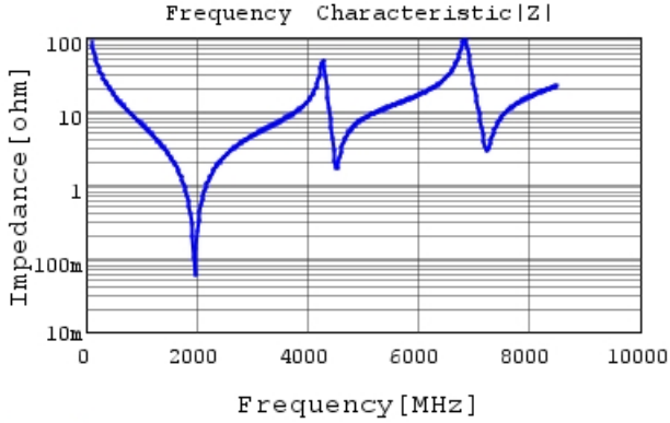
GQM1875C2E180GB12 |Z| DC0V, 25degC
