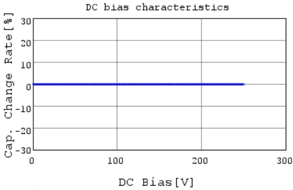
GQM1875C2E180GB12 C-DC bias capchange, 25.0c
