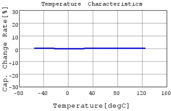
GQM1875C2E180GB12 C-Temp. capchange, DCOV, 1
