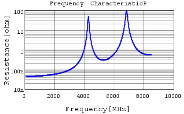
GQM1875C2E180GB12 R DC0V, 25degC
