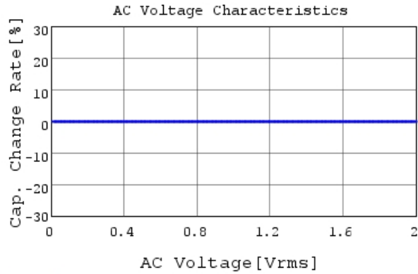
GQM1875C2E180GB12 C-AC Voltage capchange, DC
