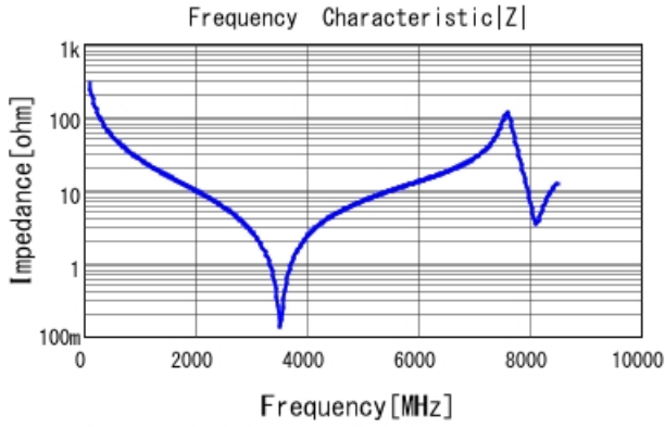
GQM1875C2E5R6CB12 |Z| DCOV, 25degC
