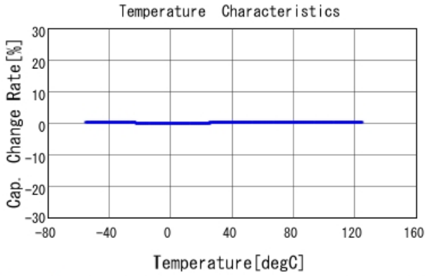
GQM1875C2E5R6CB12 C-Temp. capchange, DCOV, AC1Vrms
