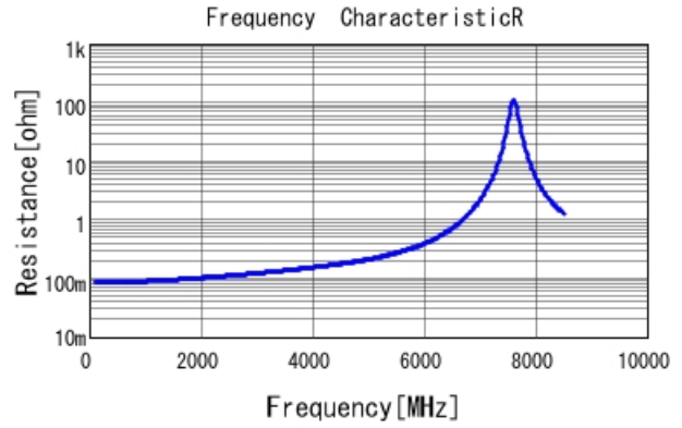
GQM1875C2E5R6CB12 R DCOV, 25degC
