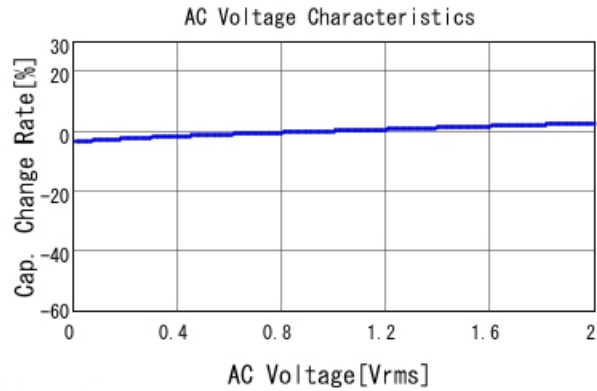
GCM188R71H154KA64 C-AC Voltage capchange, DCOV, 25
