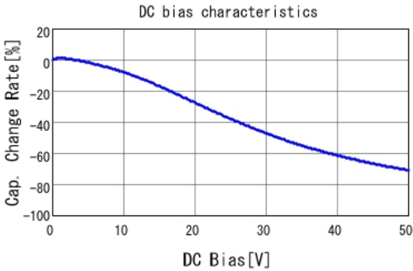
GCM188R71H154KA64 C-DC bias capchange, 25.0degC, A
