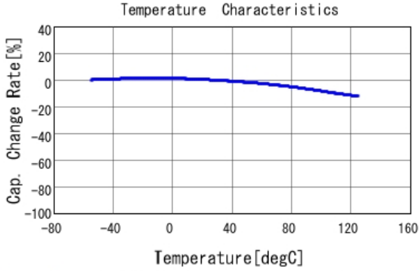
GCM188R71H154KA64 C-Temp. capchange, DC0.0V, AC1.C
