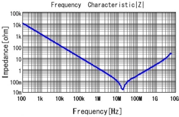
GCM188R71H154KA64 |Z| DCOV, 25degC
