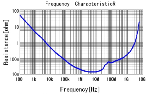
GCM188R71H154KA64 R DCOV, 25degC
