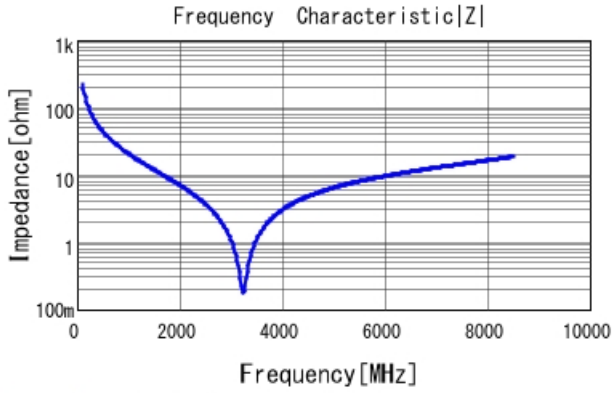
GJM1555C1H7R0DB01 |Z| DCOV, 25degC
