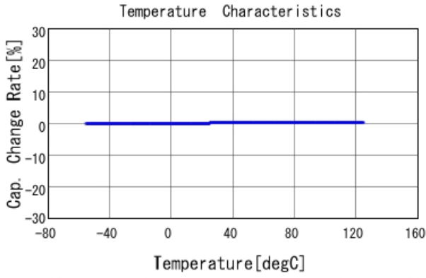
GJM1555C1H7R0DB01 C-Temp. capchange, DC0V, AC1Vrms
