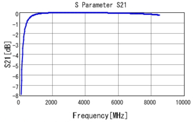
GJM1555C1H7R0DB01 S21 DC0V, 25degC
