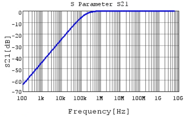
GRM033R71E103KE14 S21 DC0V,25degC
