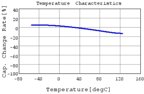
GRM033R71E103KE14 C-Temp. capchange, DC0.0V,
