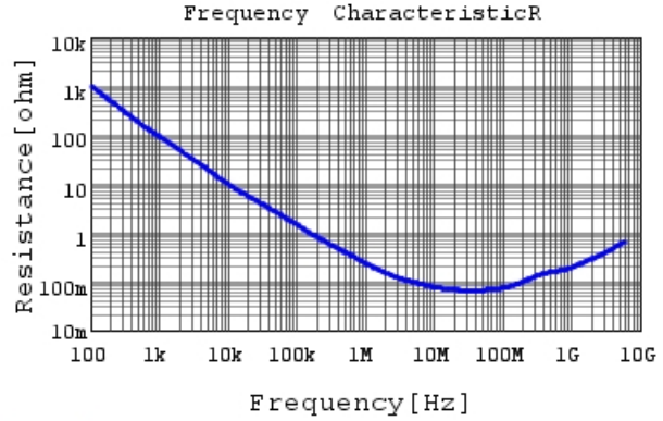
GRM033R71E103KE14 R DCOV, 25degC
