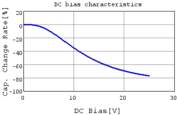
GRM033R71E103KE14 C-DC bias capchange, 25.0c
