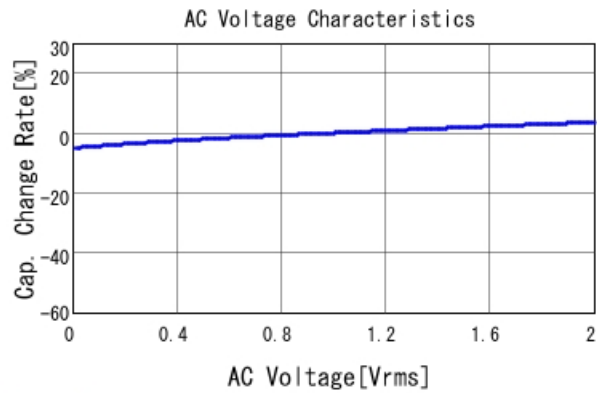
GCJ219R71E474KA12 C-AC Voltage capchange, DCOV, 25
