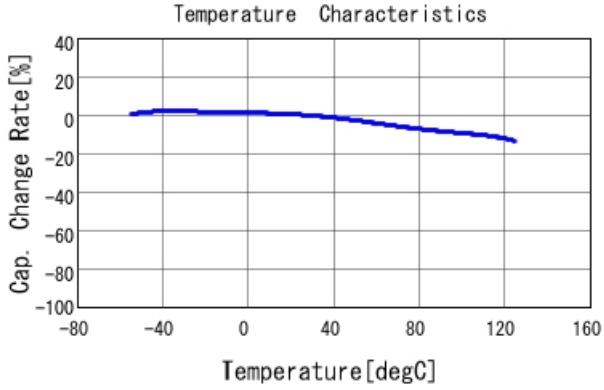
GCJ219R71E474KA12 C-Temp. capchange, DC0.0V, AC1.C
