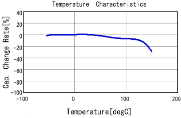
GCJ31CL8YA824KA01 C-Temp. capchange, DC0.0V, AC1.C
