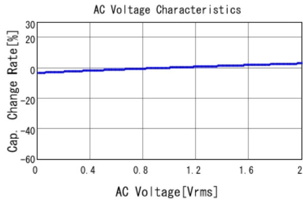
GCJ31CL8YA824KA01 C-AC Voltage capchange, DCOV, 25
