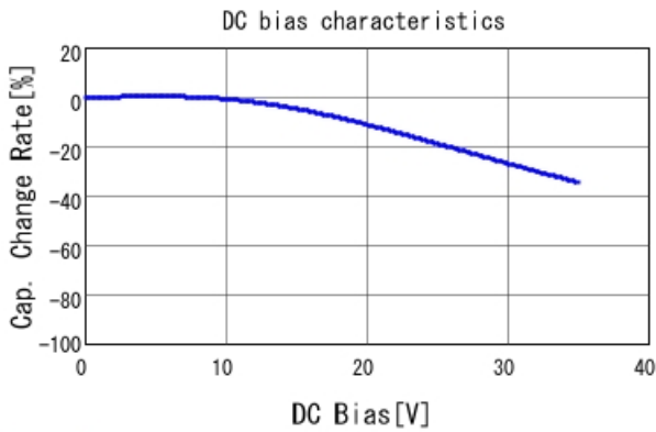
GCJ31CL8YA824KA01 C-DC bias capchange, 25.0degC, A
