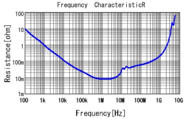
GCJ31CL8YA824KA01 R DCOV, 25degC
