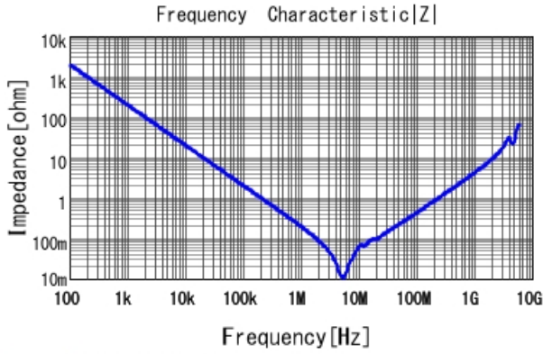
GCJ31CL8YA824KA01 |Z| DCOV, 25degC
