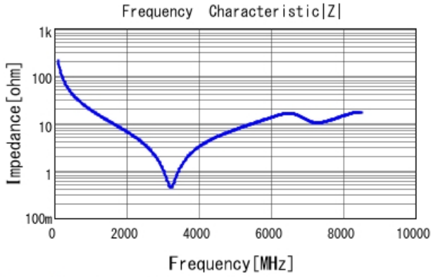
GRM1555C2A7R5DA01 |Z| DCOV, 25degC
