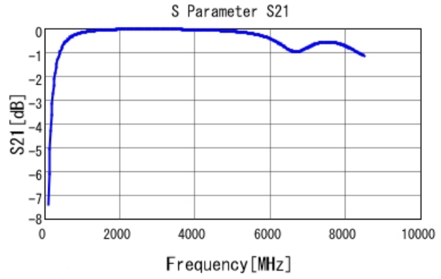
GRM1555C2A7R5DA01 S21 DC0V, 25degC
