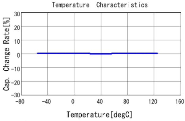
GRM1555C2A7R5DA01 C-Temp. capchange, DC0V, AC1Vrms
