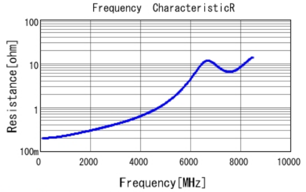
GRM1555C2A7R5DA01 R DCOV, 25degC
