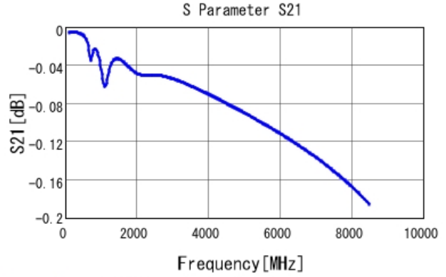
GCM1555G1H681JA16 S21 DCOV, 25degC
