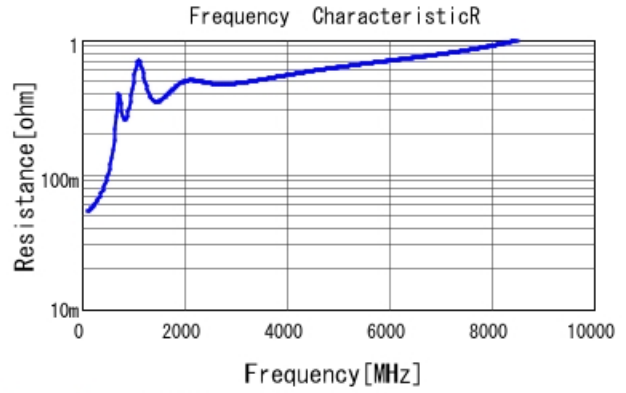
GCM1555G1H681JA16 R DCOV, 25degC
