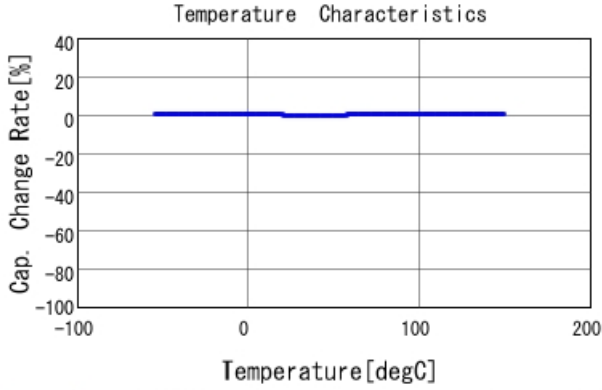
GCM1555G1H681JA16 C-Temp. capchange, DCOV, AC1Vrms
