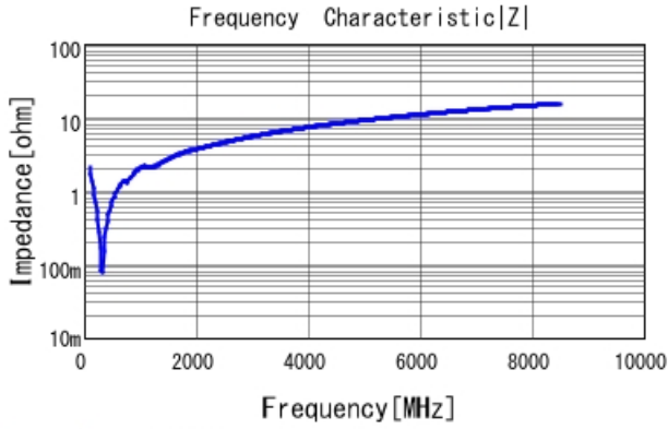
GCM1555G1H681JA16 |Z| DCOV, 25degC
