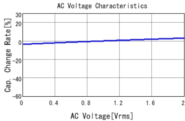
GCJ21BR71E334KA01 C-AC Voltage capchange, DCOV, 25
