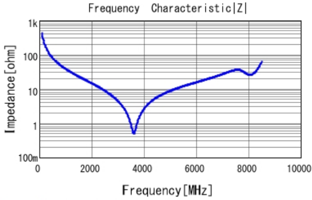
GRM1885C2A3R8WA01 |Z| DCOV, 25degC
