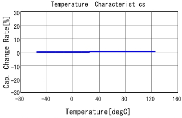
GRM1885C2A3R8WA01 C-Temp. capchange, DCOV, AC1Vrms
