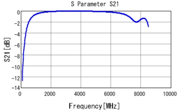
GRM1885C2A3R8WA01 S21 DCOV, 25degC
