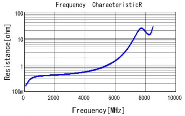
GRM1885C2A3R8WA01 R DCOV, 25degC
