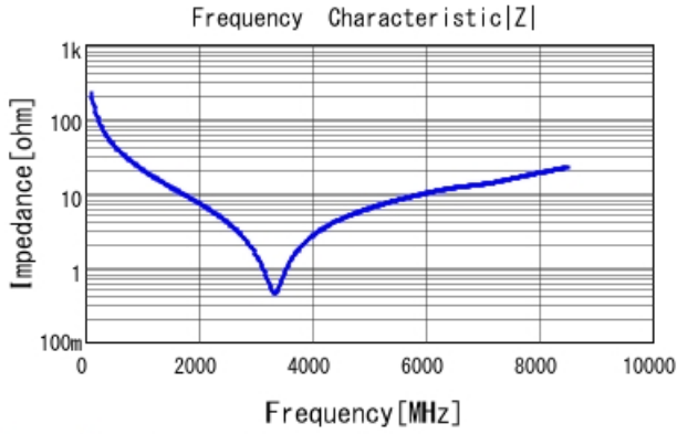
GRM1555C2A7R0CA01 |Z| DCOV, 25degC
