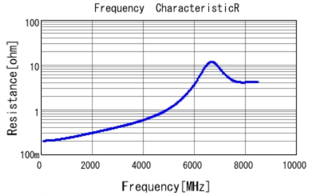
GRM1555C2A7R2CA01 R DCOV, 25degC
