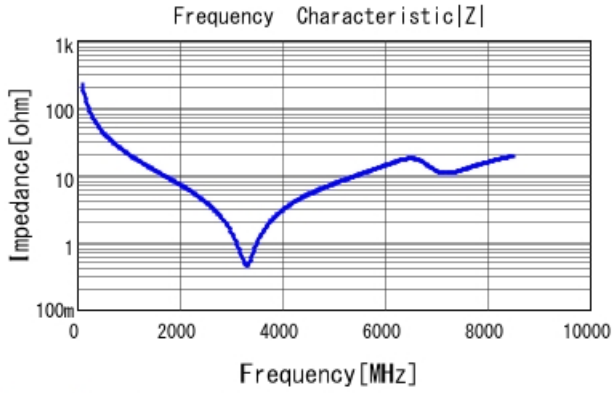
GRM1555C2A7R2CA01 |Z| DCOV, 25degC
