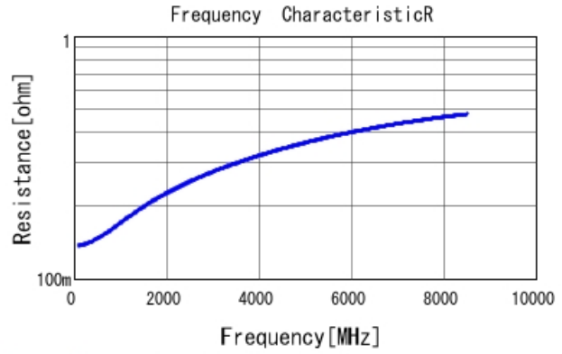
GRM0225C1C8R2DA03 R DCOV, 25degC
