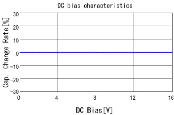
GRM0225C1C8R2DA03 C-DC bias capchange, 25.0degC, A
