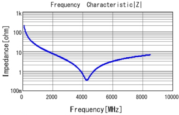
GRM0225C1C8R2DA03 |Z| DCOV, 25degC
