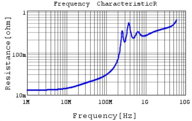
GRT1885C1H332JA02 R DCOV, 25degC
