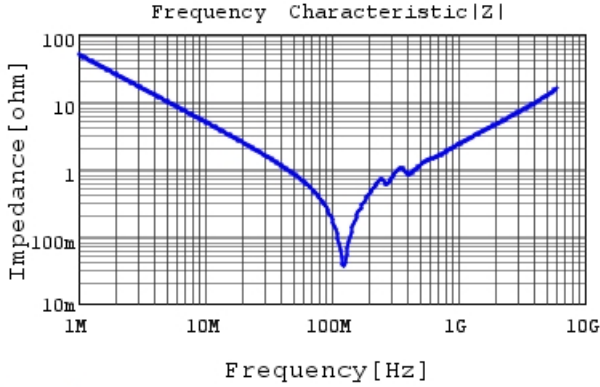
GRT1885C1H332JA02 |Z| DCOV, 25degC
