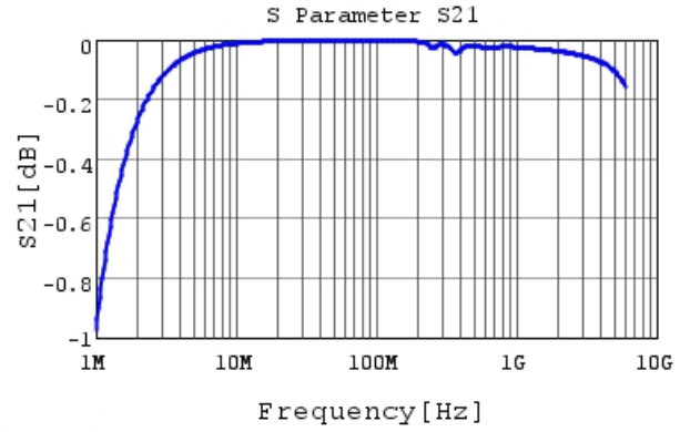
GRT1885C1H332JA02 S21 DCOV, 25degC
