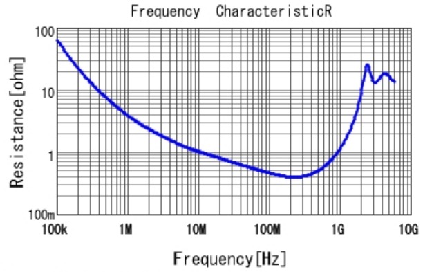
GRM31BR73A681KW01 R DCOV, 25degC
