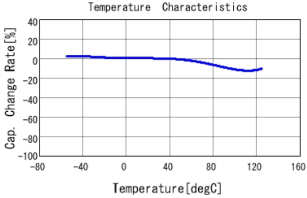
GRM31BR73A681KW01 C-Temp. capchange, DCOV, AC1Vrms
