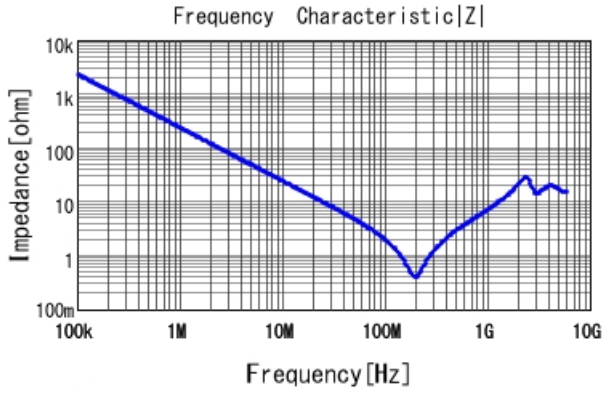
GRM31BR73A681KW01 |Z| DCOV, 25degC
