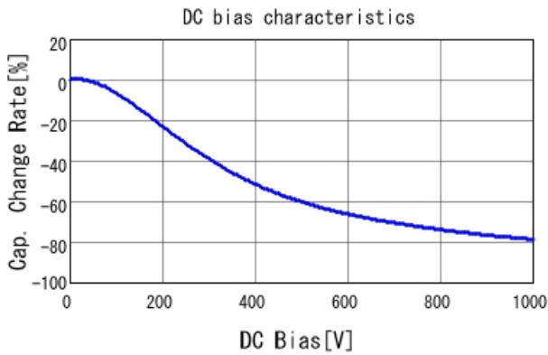
GRM31BR73A681KW01 C-DC bias capchange, 25.0degC, A
