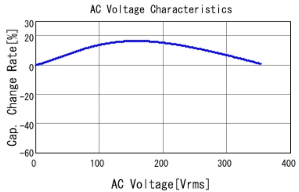
GRM31BR73A681KW01 C-AC Voltage capchange, DCOV, 25
