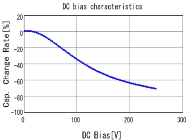
■ GRJ31CR72E333KWJ3 C-DC bias capchange, 25.0degC, AC1V
