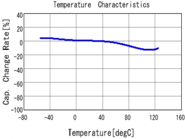
■ GRJ31CR72E333KWJ3 C-Temp. capchange, DCOV, AC1Vrms
