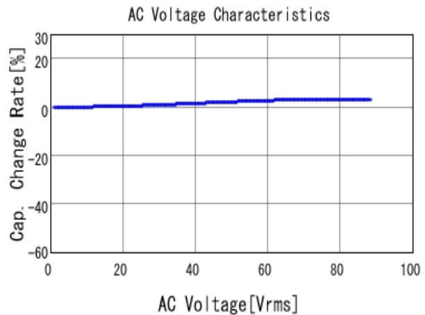
■ GRJ31CR72E333KWJ3 C-AC Voltage capchange, DCOV, 25.0d
