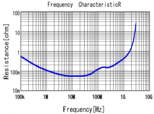
■ GRJ31CR72E333KWJ3 R DCOV, 25degC
