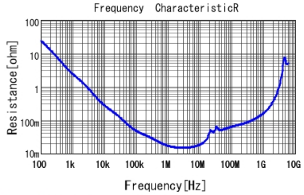
GCJ21BR71H334MA12 R DCOV, 25degC
