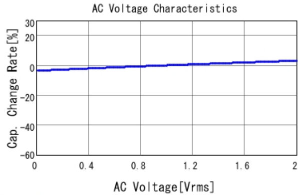
GCJ21BR71H334MA12 C-AC Voltage capchange, DCOV, 25
