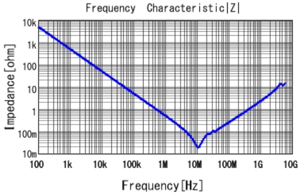
GCJ21BR71H334MA12 |Z| DCOV, 25degC
