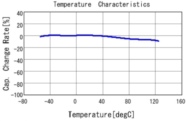
GCJ21BR71H334MA12 C-Temp. capchange, DC0.0V, AC1.C
