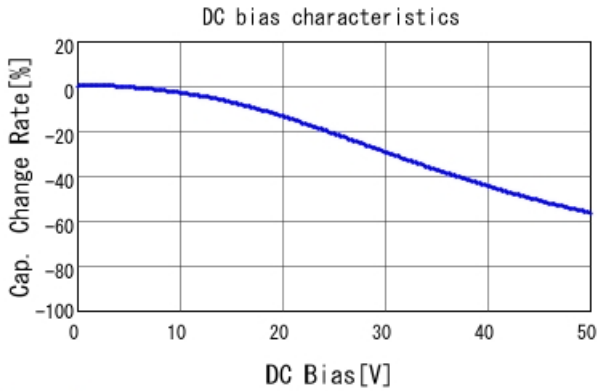
GCJ21BR71H334MA12 C-DC bias capchange, 25.0degC, A
