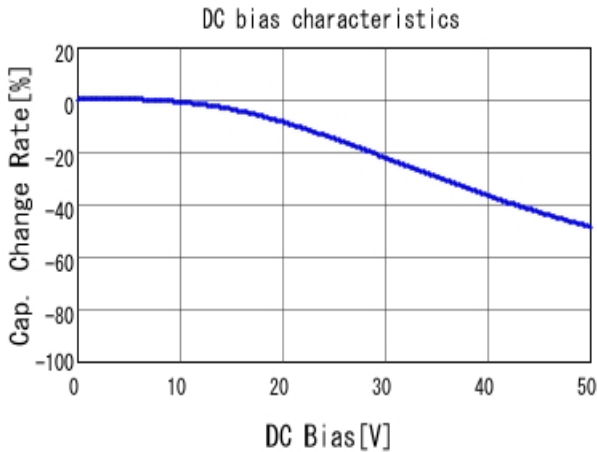
■ GCJ188R71H563KA12 C-DC bias capchange, 25.0degC, AC1.
