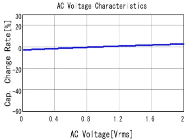
■ GCJ188R71H563KA12 C-AC Voltage capchange, DCOV, 25.0d
