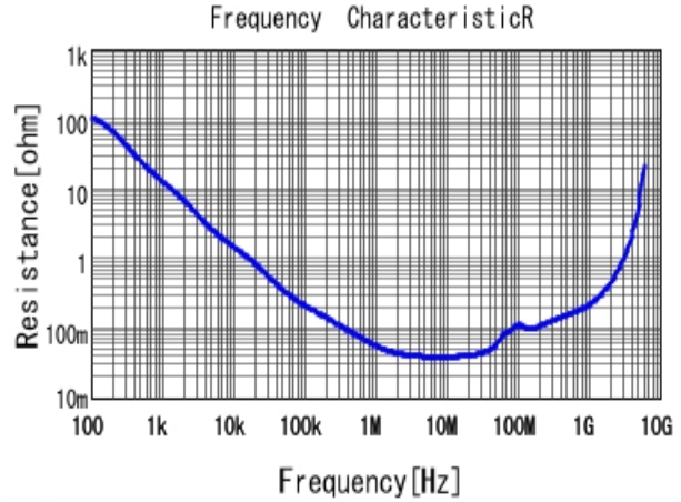
■ GCJ188R71H563KA12 R DCOV, 25degC
