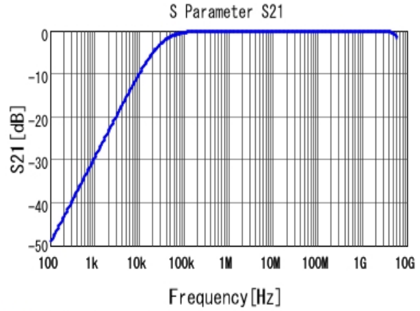
■ GCJ188R71H563KA12 S21 DCOV, 25degC
