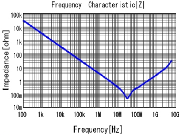
■ GCJ188R71H563KA12 |Z| DCOV, 25degC
