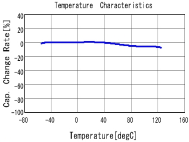
■ GCJ188R71H563KA12 C-Temp. capchange, DCO. 0V, AC1.0V rm
