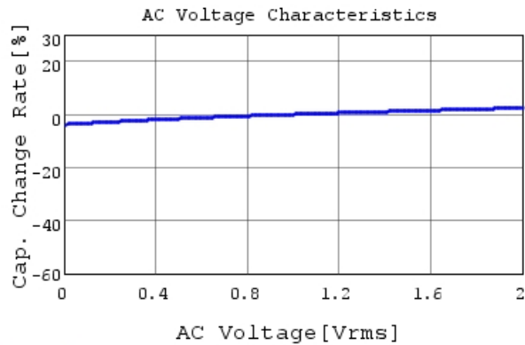
GCJ188R71H183KA01 C-AC Voltage capchange, Dc
