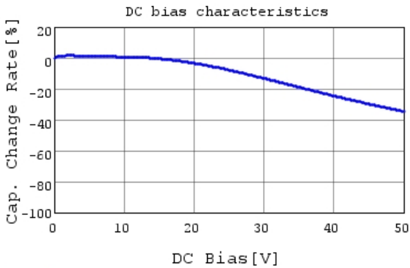
GCJ188R71H183KA01 C-DC bias capchange, 25.0c
