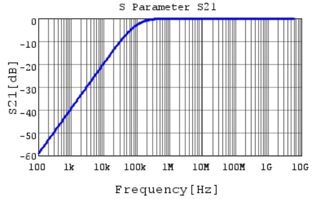
GCJ188R71H183KA01 S21 DC0V,25degC
