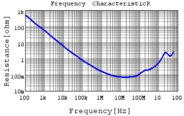
GCJ188R71H183KA01 R DCOV,25degC
