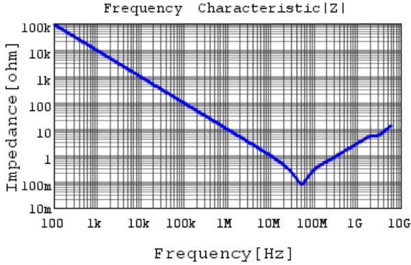
GCJ188R71H183KA01 |Z| DCOV,25degC
