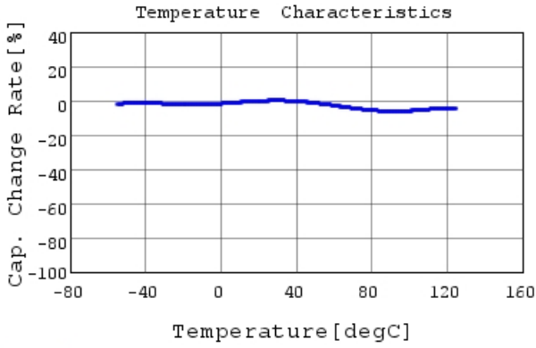
GCJ188R71H183KA01 C-Temp. capchange, DC0.0V,
