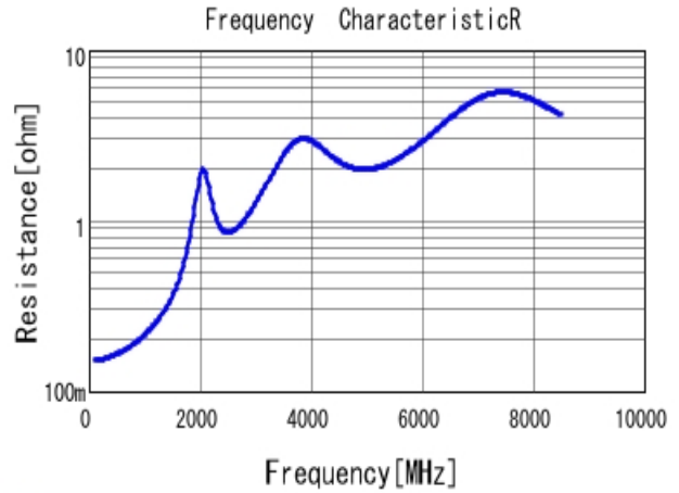
■ GRT1885C1H470JA02 R DC0V, 25degC
