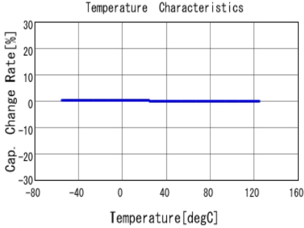
■ GRT1885C1H470JA02 C-Temp. capchange, DCOV, AC1Vrms
