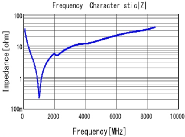
■ GRT1885C1H470JA02 |Z| DC0V, 25degC
