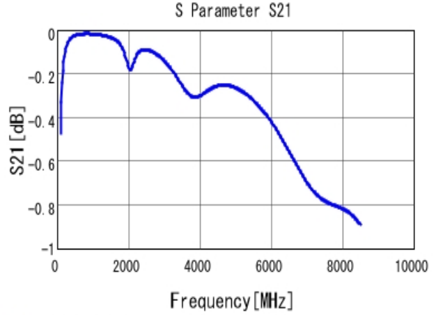
■ GRT1885C1H470JA02 S21 DCOV, 25degC
