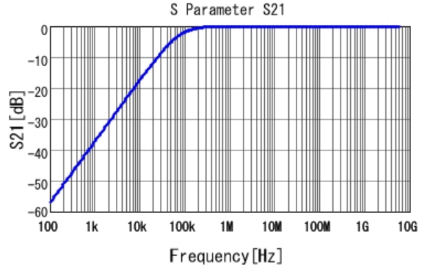
GRM155R71E223MA61 S21 DC0V, 25degC
