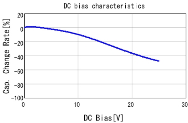
GRM155R71E223MA61 C-DC bias capchange, 25.0degC, A
