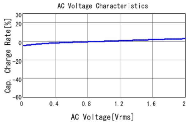
GRM155R71E223MA61 C-AC Voltage capchange, DCOV, 25
