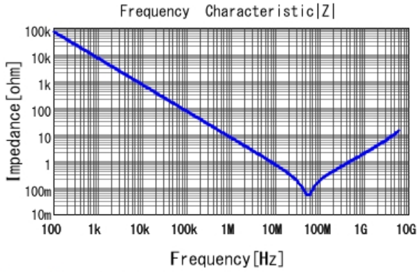
GRM155R71E223MA61 |Z| DCOV, 25degC
