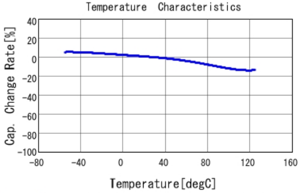
GRM155R71E223MA61 C-Temp. capchange, DC0.0V, AC1.C
