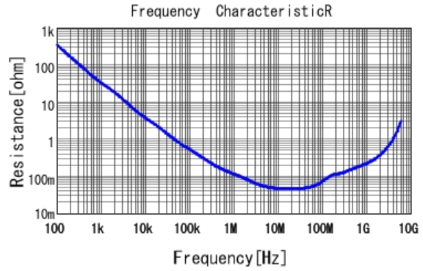
GRM155R71E223MA61 R DCOV, 25degC
