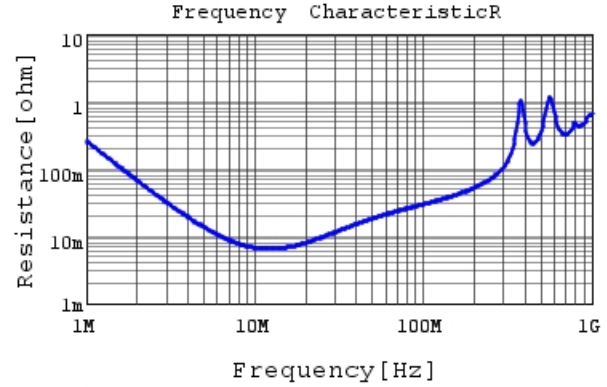
GRM21B5C2J122JWA3 R DC0V, 25degC
