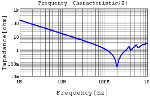
GRM21B5C2J122JWA3 |Z| DC0V, 25degC
