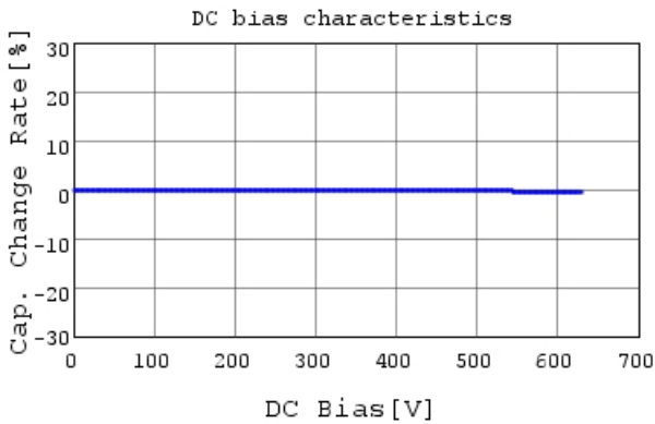
GRM21B5C2J122JWA3 C-DC bias capchange, 25.0c
