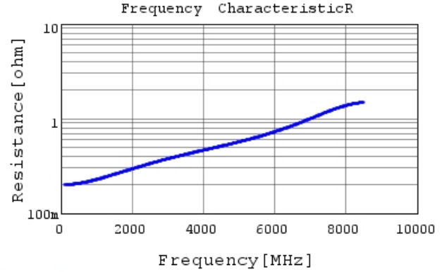
GRT0335C1H6R0DA02 R DCOV, 25degC
