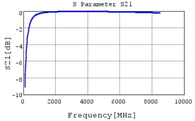
GRT0335C1H6R0DA02 S21 DCOV, 25degC
