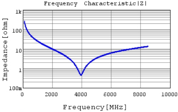
GRT0335C1H6R0DA02 |Z| DCOV, 25degC
