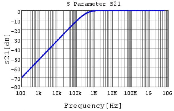
GRT033R70J472KE01 S21 DC0V, 25degC
