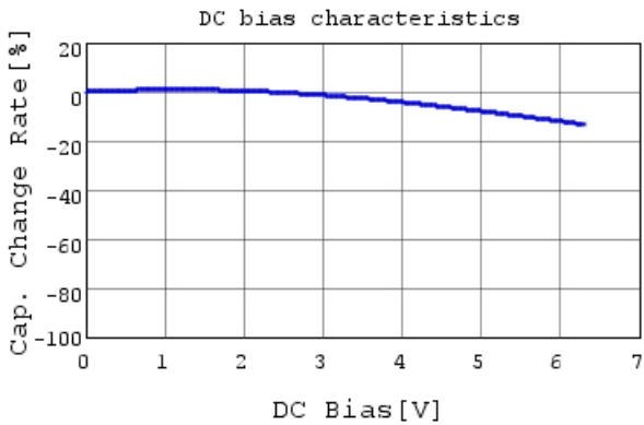
GRT033R70J472KE01 C-DC bias capchange, 25.0c
