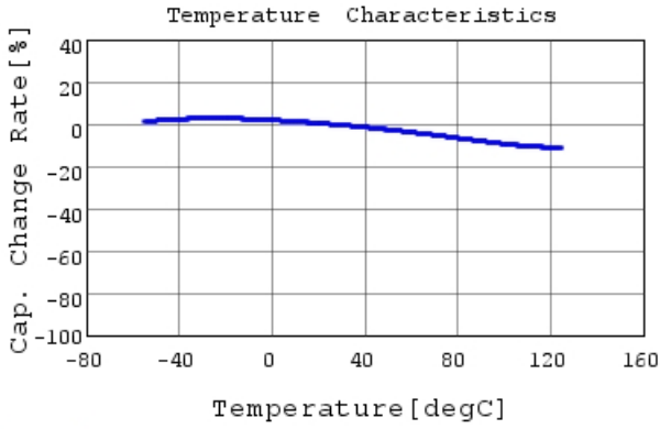
GRT033R70J472KE01 C-Temp. capchange, DC0.0V,
