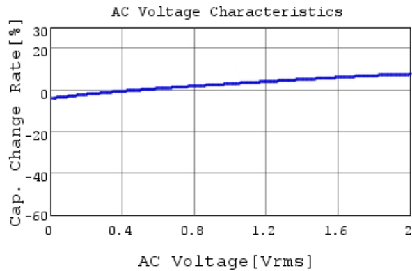
GRT033R70J472KE01 C-AC Voltage capchange, Dc
