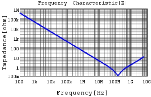
GRT033R70J472KE01 |Z| DCOV, 25degC
