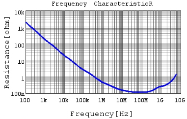
GRT033R70J472KE01 R DCOV, 25degC
