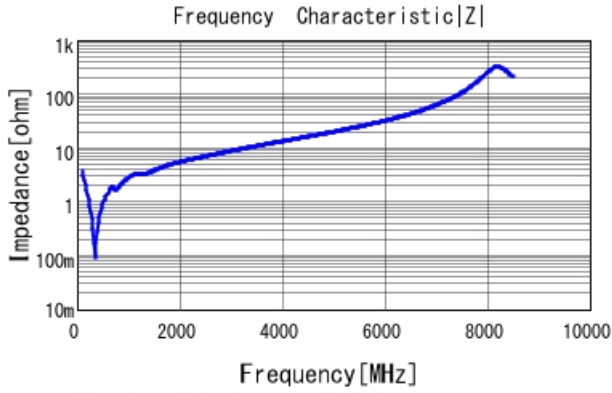
GRM1885C2A391JA01 |Z| DCOV, 25degC
