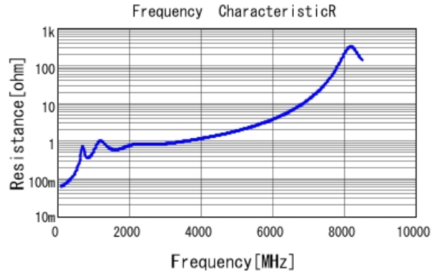
GRM1885C2A391JA01 R DCOV, 25degC
