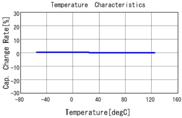
GRM1885C2A391JA01 C-Temp. capchange, DCOV, AC1Vrms
