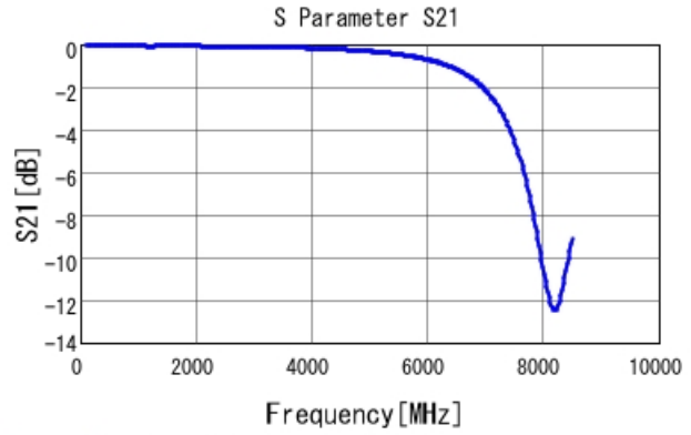
GRM1885C2A391JA01 S21 DCOV, 25degC
