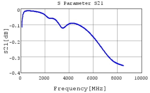
GRM0335C1E101JA01 S21 DCOV, 25degC
