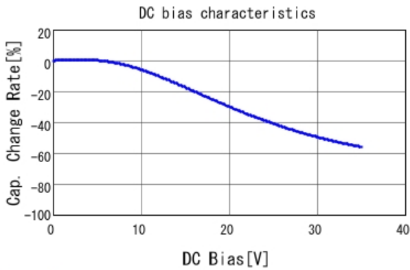
GCJ21BL8YA474KA01 C-DC bias capchange, 25.0degC, A
