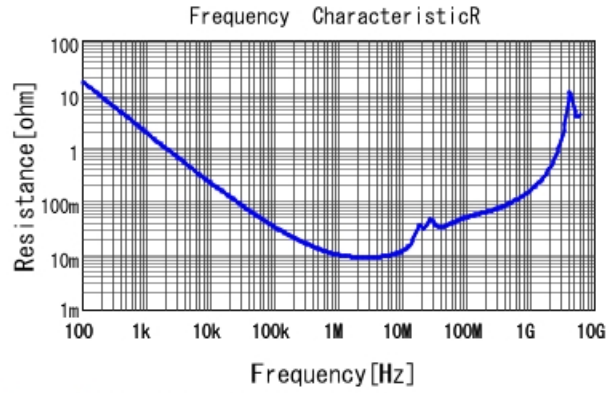
GCJ21BL8YA474KA01 R DCOV, 25degC
