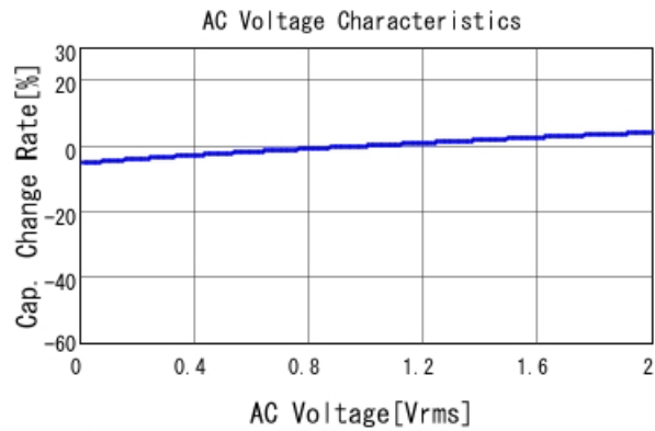
GCJ21BL8YA474KA01 C-AC Voltage capchange, DCOV, 25
