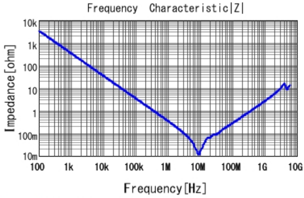
GCJ21BL8YA474KA01 |Z| DCOV, 25degC
