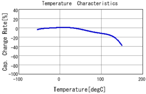
GCJ21BL8YA474KA01 C-Temp. capchange, DC0.0V, AC1.C
