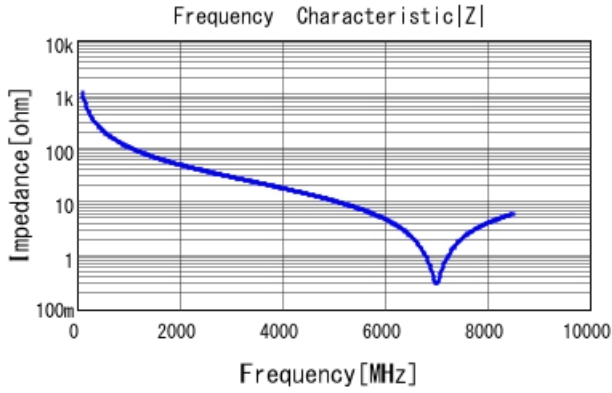
GJM1555C1H1R5BB01 |Z| DC0V, 25degC
