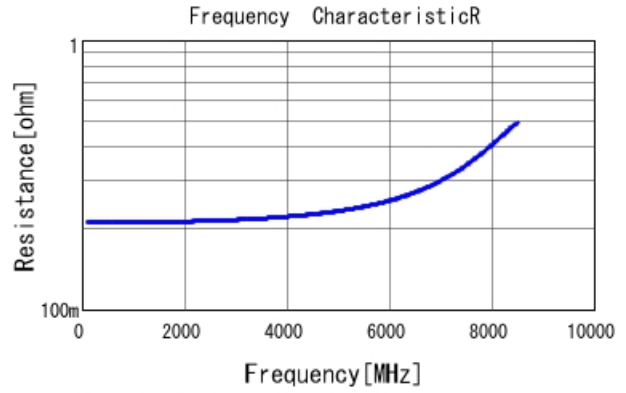
GJM1555C1H1R5BB01 R DC0V, 25degC
