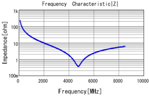
GRM0225C1E6R7DA03 |Z| DCOV, 25degC
