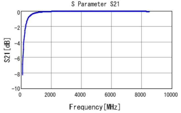
GRM0225C1E6R7DA03 S21 DC0V, 25degC
