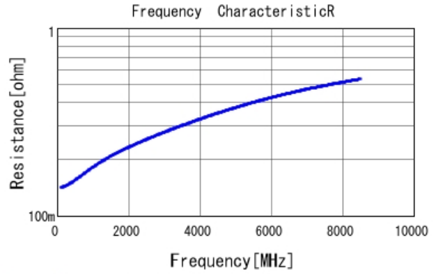
GRM0225C1E6R7DA03 R DCOV, 25degC
