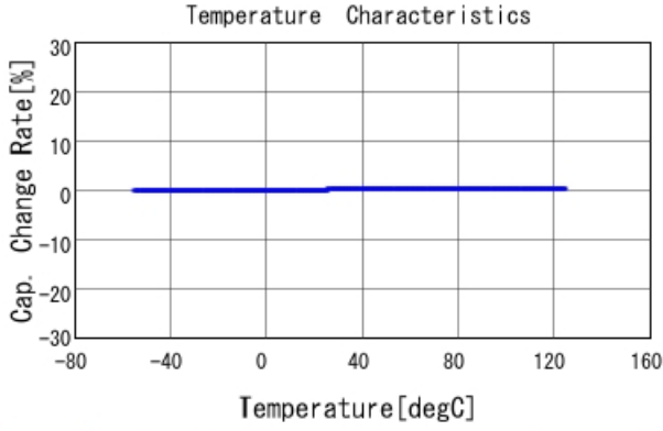
GRM0225C1E6R7DA03 C-Temp. capchange, DC0V, AC1Vrms
