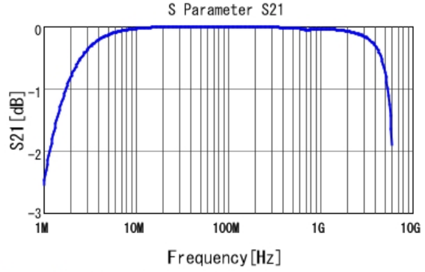
GRM3195C2A182JA01 S21 DCOV, 25degC
