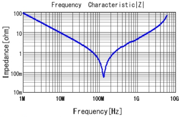
GRM3195C2A182JA01 |Z| DCOV, 25degC
