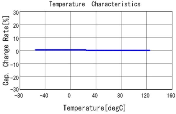
GRM3195C2A182JA01 C-Temp. capchange, DCOV, AC1Vrms
