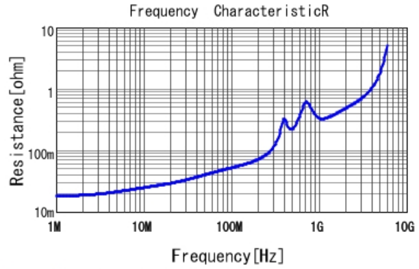
GRM3195C2A182JA01 R DCOV, 25degC
