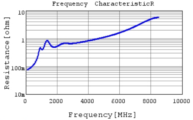
GCM1555C1H391JA16 R DC0V, 25degC
