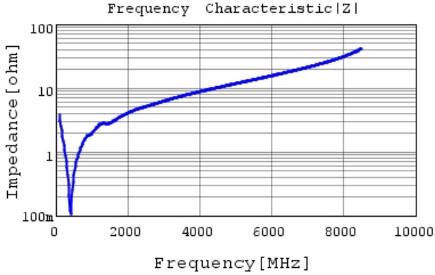
GCM1555C1H391JA16 |Z| DC0V, 25degC
