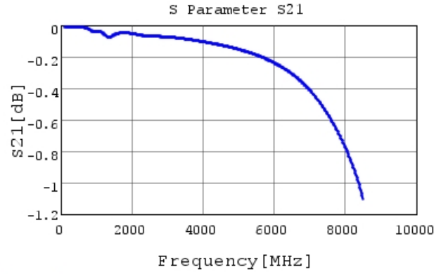
GCM1555C1H391JA16 S21 DCOV, 25degC
