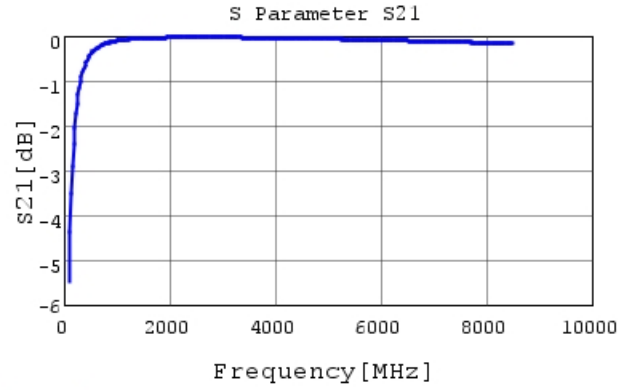
GRT0335C1H100JA02 S21 DCOV, 25degC
