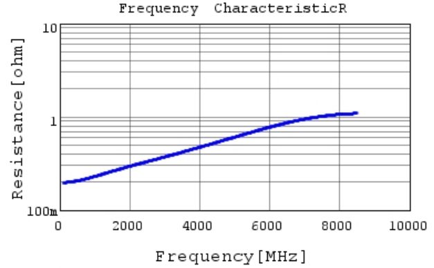
GRT0335C1H100JA02 R DCOV, 25degC
