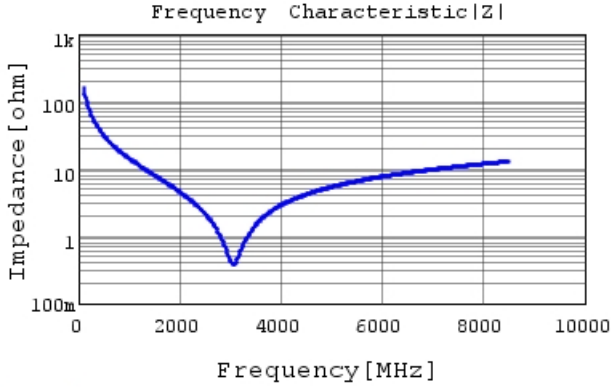
GRT0335C1H100JA02 |Z| DCOV, 25degC
