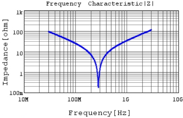
RDE5C3A560J2M1H03A |Z| DC0V, 25degC
