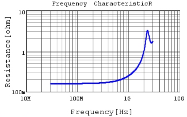
RDE5C3A560J2M1H03A R DC0V, 25degC
