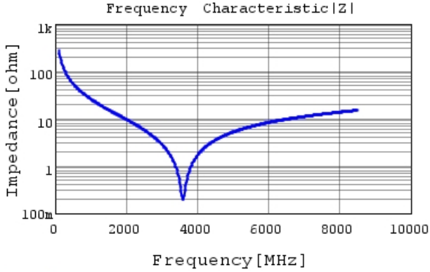
GCQ1555C1H5R7DB01 |Z| DC0V, 25degC
