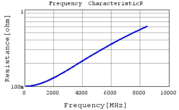
GCQ1555C1H5R7DB01 R DC0V, 25degC
