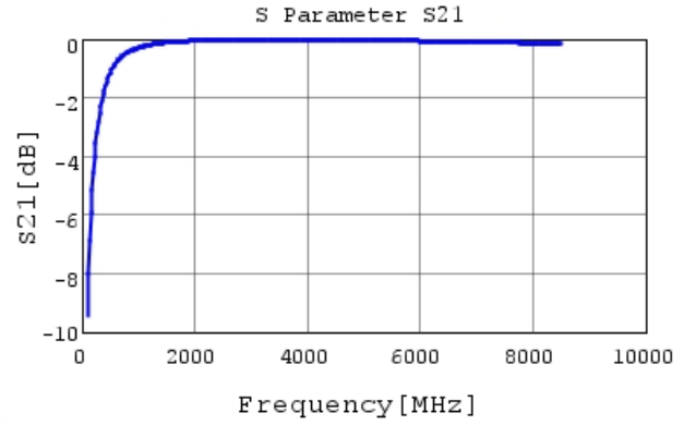
GCQ1555C1H5R7DB01 S21 DCOV, 25degC
