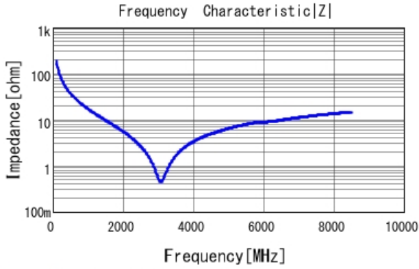
GRM1555C2A8R3BA01 |Z| DCOV, 25degC
