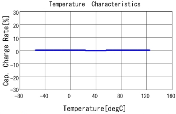
GRM1555C2A8R3BA01 C-Temp. capchange, DCOV, AC1Vrms
