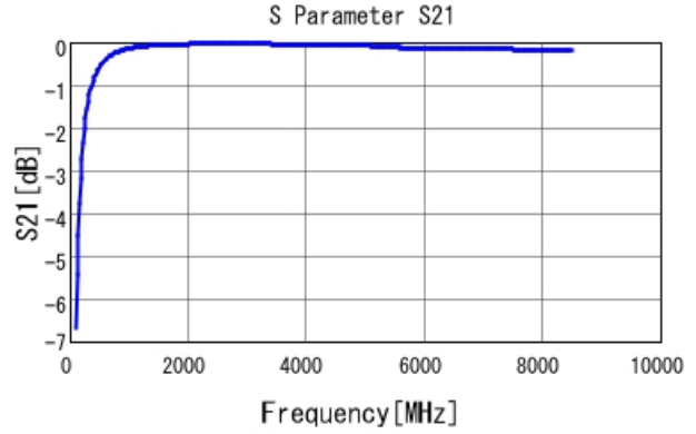
GRM1555C2A8R3BA01 S21 DCOV, 25degC
