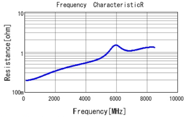
GRM1555C2A8R3BA01 R DCOV, 25degC
