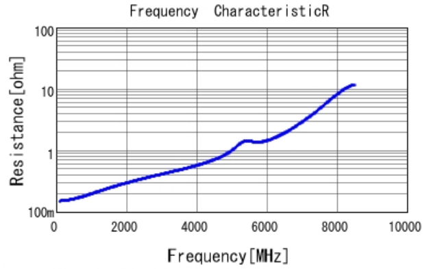
GRM1555C1H9R9CA01 R DCOV, 25degC
