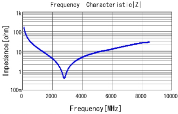
GRM1555C1H9R9CA01 |Z| DCOV, 25degC
