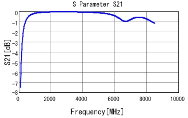
GRM1555C2A7R4BA01 S21 DC0V, 25degC
