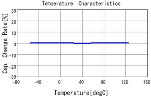
GRM1555C2A7R4BA01 C-Temp. capchange, DC0V, AC1Vrms
