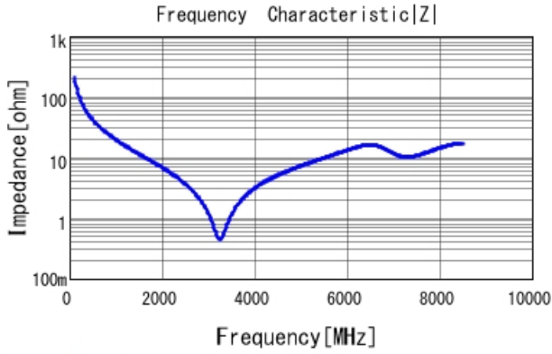
GRM1555C2A7R4BA01 |Z| DCOV, 25degC
