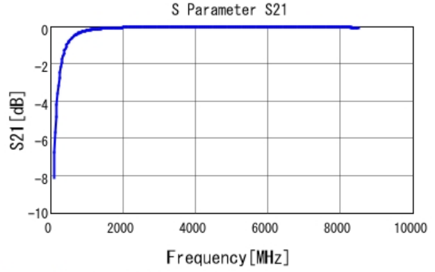
GRM0225C1E6R8BA03 S21 DC0V, 25degC
