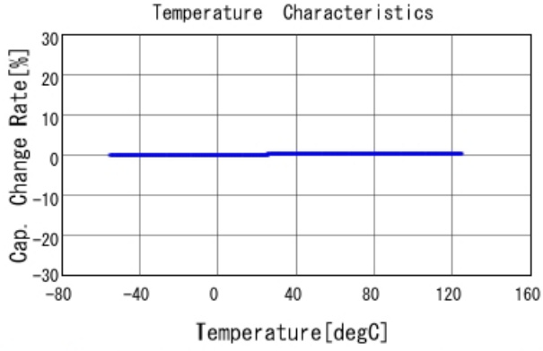
GRM0225C1E6R8BA03 C-Temp. capchange, DC0V, AC1Vrms
