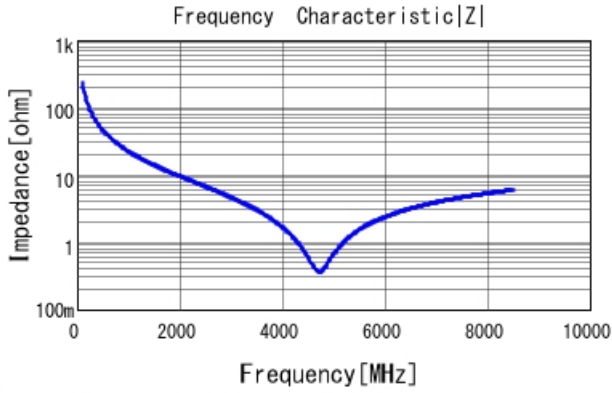
GRM0225C1E6R8BA03 |Z| DCOV, 25degC
