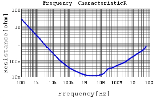
GRT155R61A474KE01 R DCOV, 25degC
