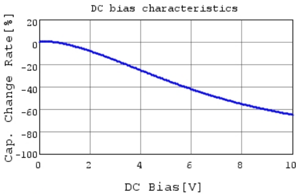
GRT155R61A474KE01 C-DC bias capchange, 25.0c
