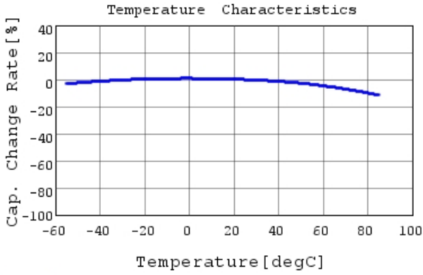
GRT155R61A474KE01 C-Temp. capchange, DC0.0V,
