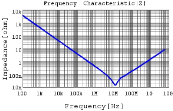
GRT155R61A474KE01 |Z| DCOV, 25degC
