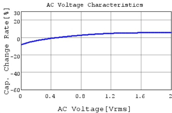
GRT155R61A474KE01 C-AC Voltage capchange, DC
