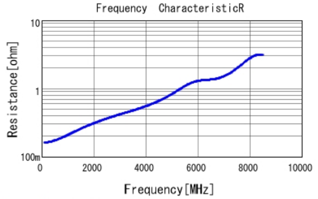
GRM1555C1H9R7BA01 R DCOV, 25degC
