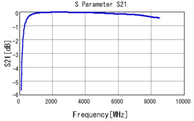
GRM1555C1H9R7BA01 S21 DCOV, 25degC
