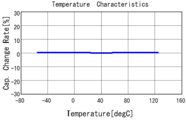
GRM1555C1H9R7BA01 C-Temp. capchange, DCOV, AC1Vrms
