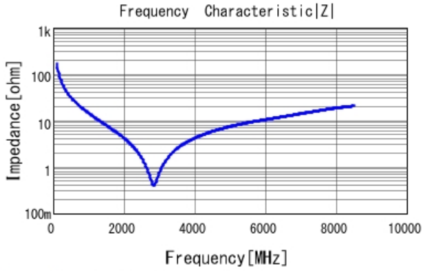
GRM1555C1H9R7BA01 |Z| DCOV, 25degC
