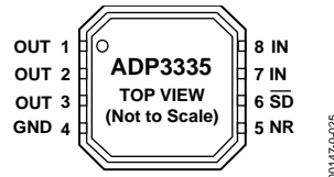
Figure 3. 8-Lead MSOP
