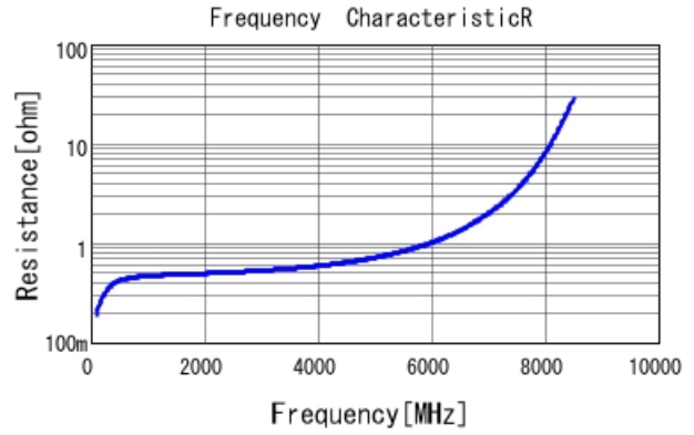
GRM1885C2A3R4WA01 R DCOV, 25degC
