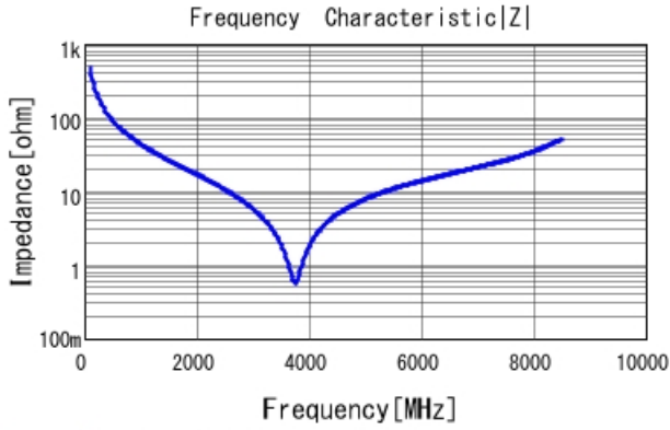
GRM1885C2A3R4WA01 |Z| DCOV, 25degC
