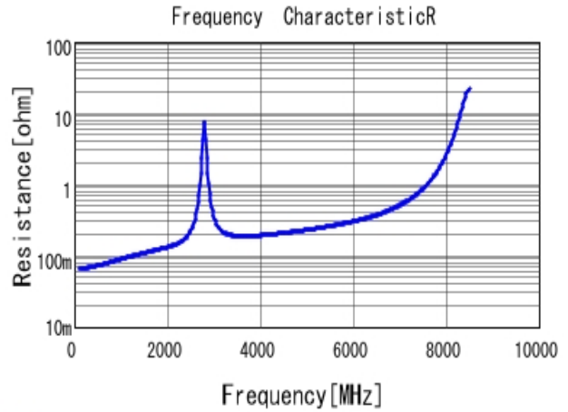
■ GQM1885C1H220JB01 R DC0V, 25degC
