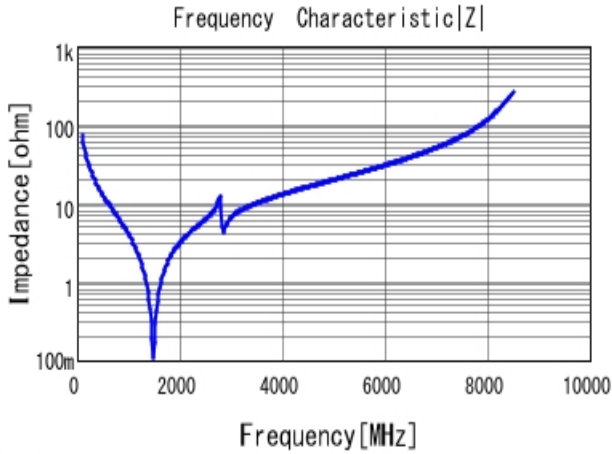
■ GQM1885C1H220JB01 |Z| DC0V, 25degC
