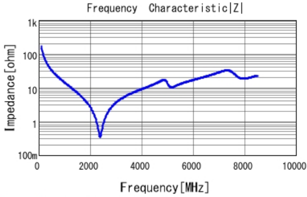
GRM1885C1H9R2BA01 |Z| DCOV, 25degC
