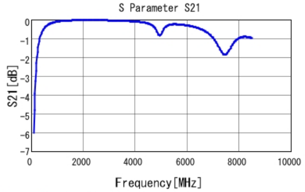
GRM1885C1H9R2BA01 S21 DCOV, 25degC
