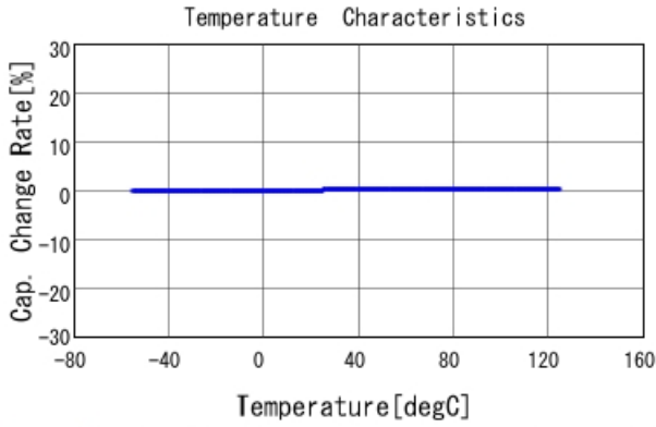
GRM1885C1H9R2BA01 C-Temp. capchange, DCOV, AC1Vrms
