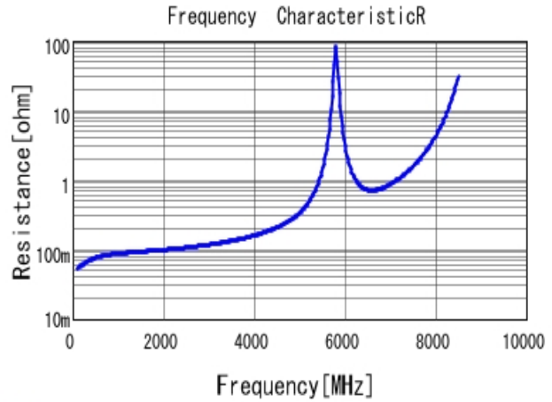
■ GQM2195C2A6R2DB01 R DC0V, 25degC
