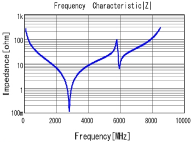
■ GQM2195C2A6R2DB01 |Z| DC0V, 25degC
