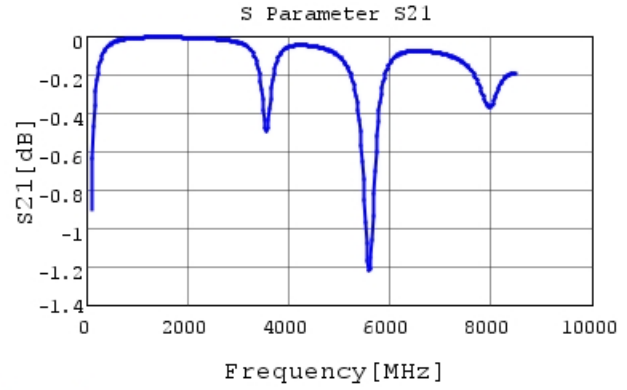
GCQ1555C1H330FB01 S21 DCOV, 25degC
