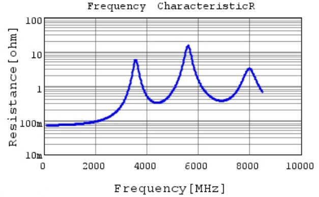
GCQ1555C1H330FB01 R DC0V, 25degC
