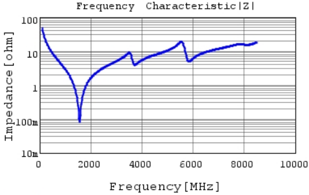
GCQ1555C1H330FB01 |Z| DC0V, 25degC
