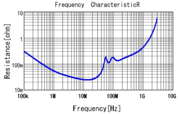
■ GA243DR7E2473MW01 R DCOV, 25degC
