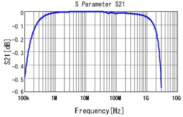
■ GA243DR7E2473MW01 S21 DCOV, 25degC
