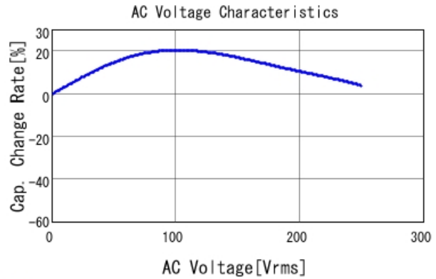
■ GA243DR7E2473MW01 C-AC Voltage capchange, DCOV, 25.0d
