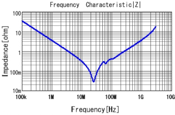
■ GA243DR7E2473MW01 |Z| DCOV, 25degC
