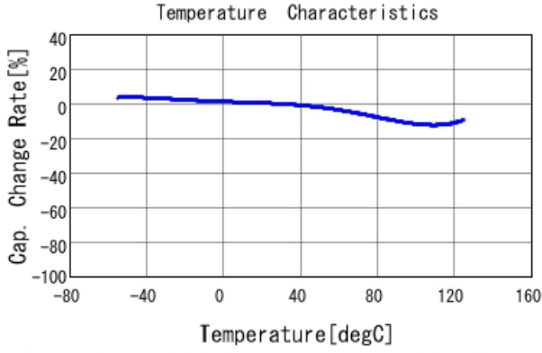
■ GA243DR7E2473MW01 C-Temp. capchange, DCOV, AC1Vrms
