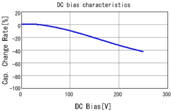
■ GA243DR7E2473MW01 C-DC bias capchange, 25.0degC, AC1V
